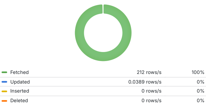
Read/Write ratio ⓘ 📄
