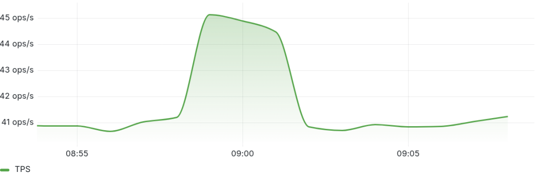
Read/Write ratio ⓘ 📄
